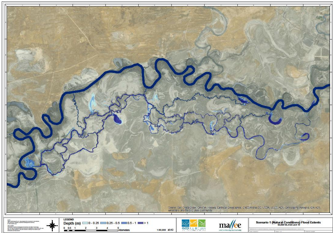
Figure 8-2a. Wallpolla Island floodplain inundation at flows of 60,000 ML/d (Water Technology, 2014)
