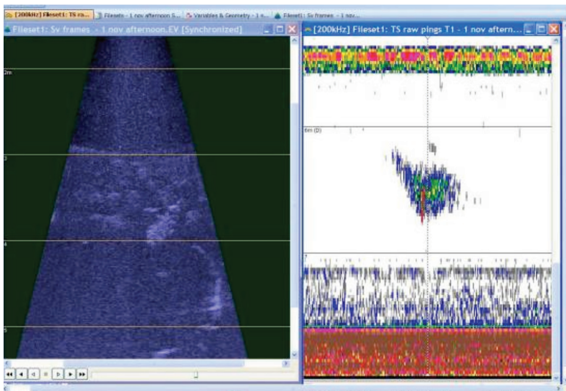
Figure 4: Echogram showing a school of fish (encircled in red) swimming out of the fishway exit channel at Lock 10 fishway and detected by the split-beam system (window on right) and the DIDSON system (window on left). The red shape around the selected single targets in the right-hand window indicates the targets were selected as a fish track by the software.
