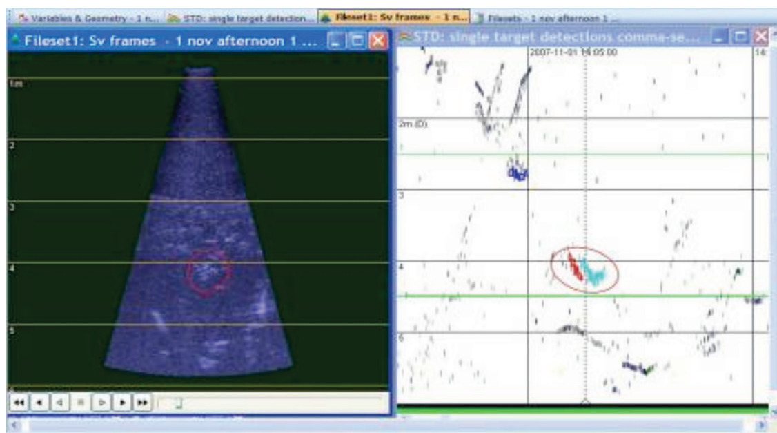
Figure 5: Echogram showing a school of fish detected swimming out of the fishway exit channel at Lock 10 fishway by the DIDSON system. The window on the left shows the acoustic system image the window on the right shows the single targets and two fish tracks (red and blue shapes around targets).
