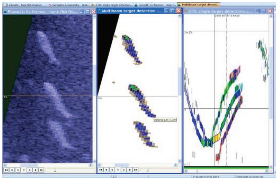
Figure 7: A DIDSON echogram showing the three tank fish detected swimming across the tank (left window), the fish extracted from background noise in the multibeam target detection variable with the central fish manually measured (centre window) and the single target detection variable with fish tracks (right window). The central window shows the multibeam target detection variable and the measurement of the second fish.
