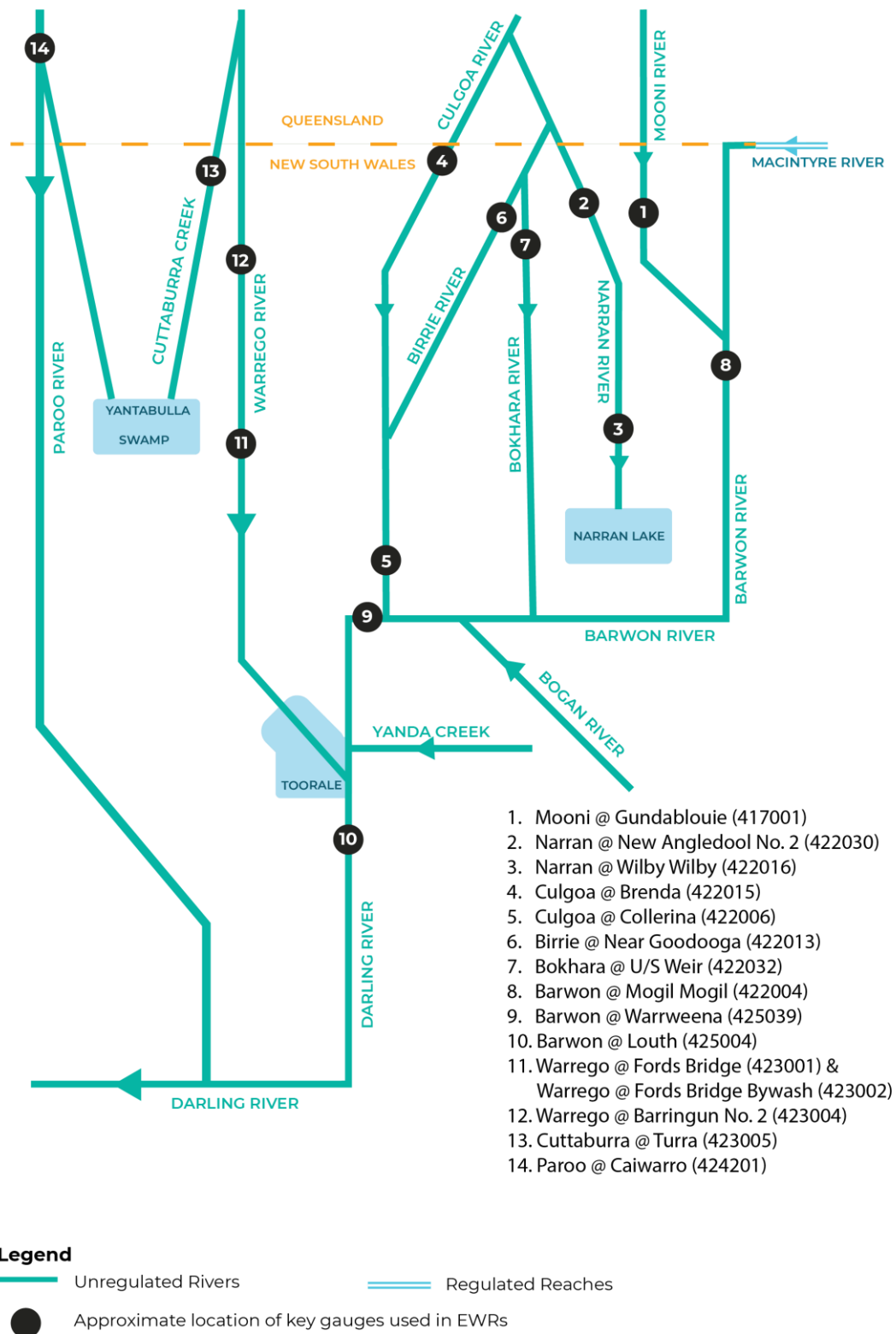
Figure 7 A schematic diagram of the main watercourses and key gauges referred to in the Intersecting Streams Long Term Water Plan
