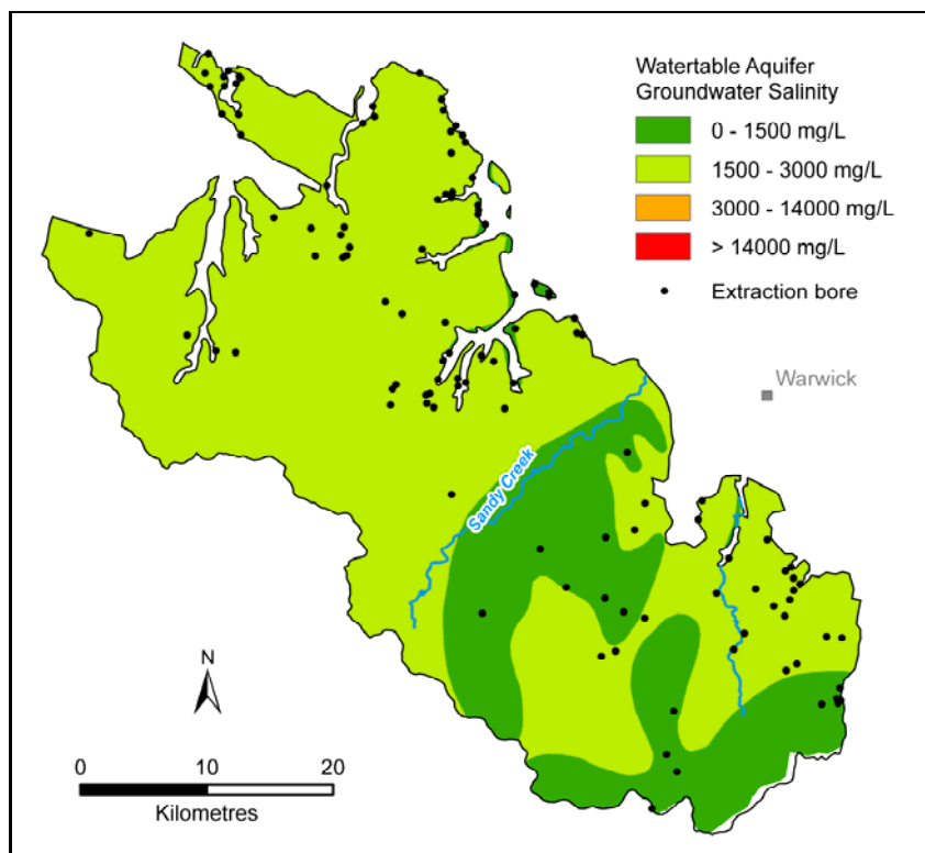
Figure 8. Condamine Fractured Rock SDL area watertable aquifer salinity distribution, from the shallow salinity layer of the MDBA Basin in a Box dataset (MDBA, 2000)
