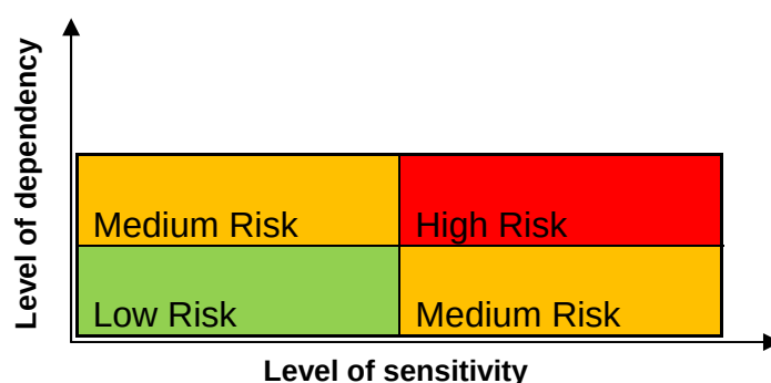
Figure 4. Key environmental asset – groundwater dependency versus sensitivity
