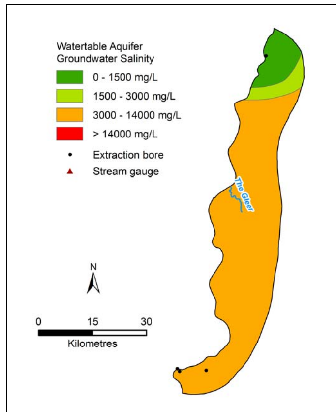
Figure 15. St George Alluvium: Moonie SDL area watertable aquifer salinity distribution, from the shallow salinity layer of the MDBA Basin in a Box dataset (MDBA, 2000)
