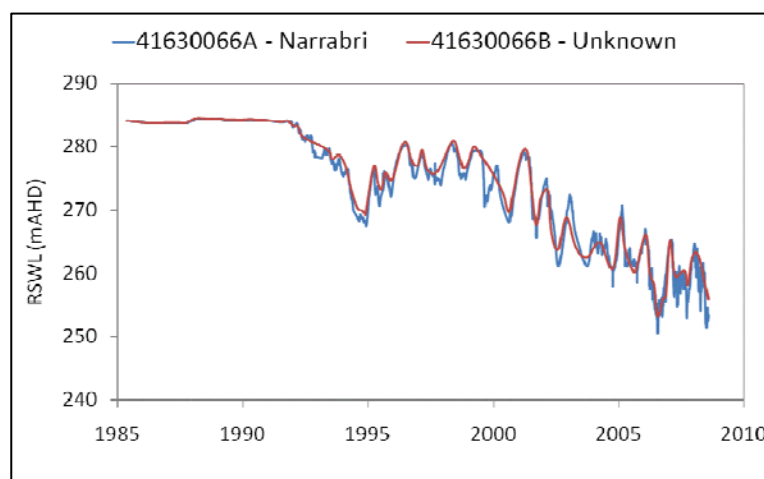
Figure 5. Hydrograph for bores screening the shallow and deep alluvial aquifers
