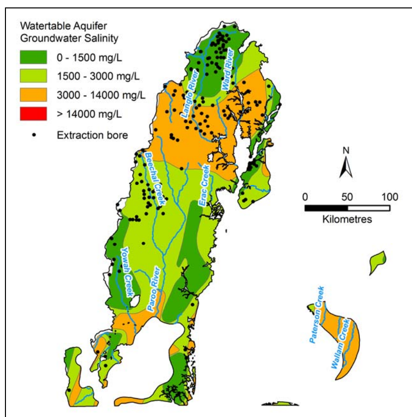
Figure 13. Sediments Above GAB: Warrego-Paroo-Nebine watertable aquifer salinity distribution, from the shallow salinity layer of the MDBA Basin in a Box dataset (MDBA, 2000)
