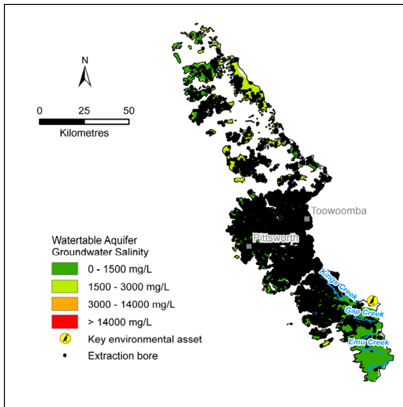
Figure 2. Upper Condamine Basalts watertable aquifer salinity distribution, from the shallow salinity layer of the MDBA Basin in a Box dataset (MDBA, 2000)
