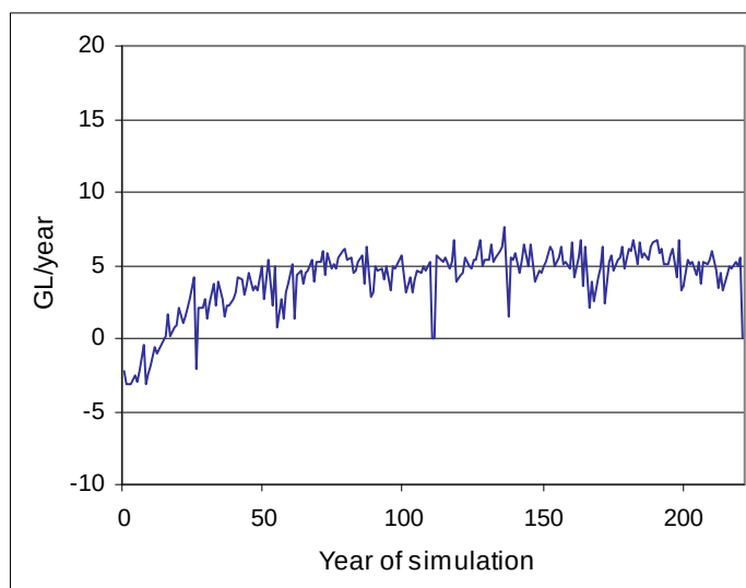
Figure 7. Annual net river loss of the Dumaresq River under a historical climate and 2004/2005 level of groundwater development (from Welsh, 2007)
