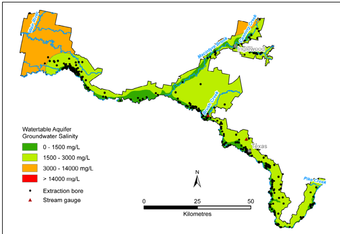
Figure 6. Border Rivers Alluvium (Qld) SDL area watertable aquifer salinity distribution, from the shallow salinity layer of the MDBA Basin in a Box dataset (MDBA, 2000)
