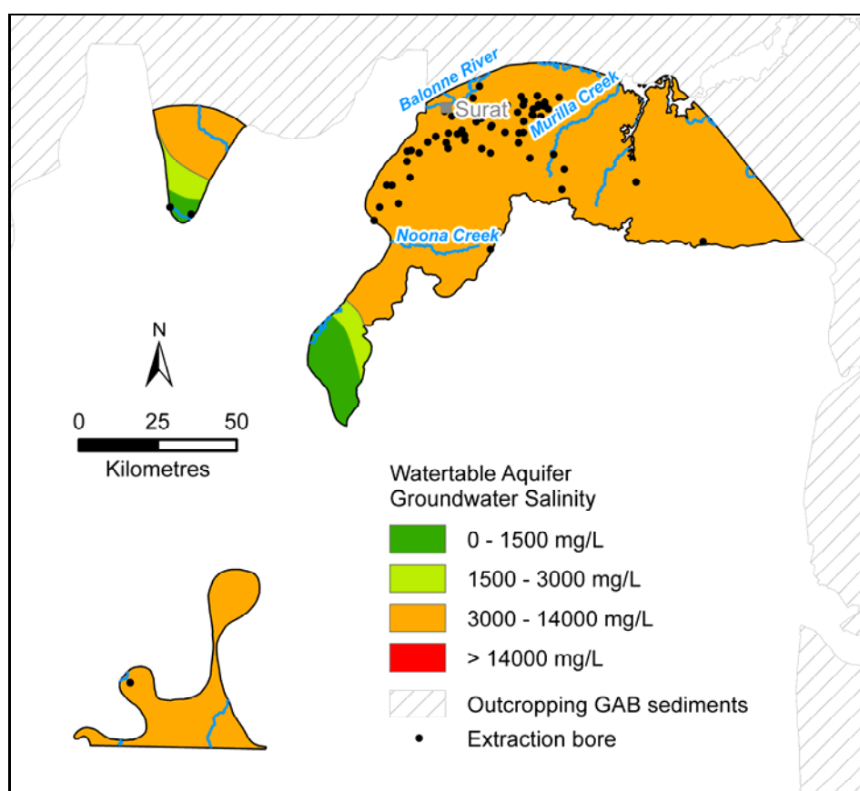
Figure 11. Sediments Above GAB: Condamine-Balonne watertable aquifer salinity distribution, from the shallow salinity layer of the MDBA Basin in a Box dataset (MDBA, 2000)
