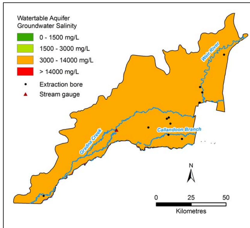
Figure 12. Sediments Above GAB: Border Rivers watertable aquifer salinity distribution, from the shallow salinity layer of the MDBA Basin in a Box dataset (MDBA, 2000)
