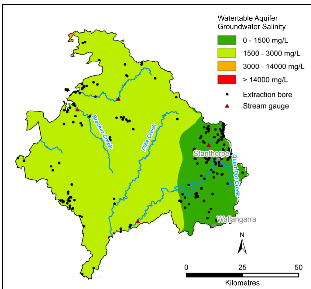
Figure 9. Border Rivers Fractured Rock SDL area watertable aquifer salinity distribution, from the shallow salinity layer of the MDBA Basin in a Box dataset (MDBA, 2000)
