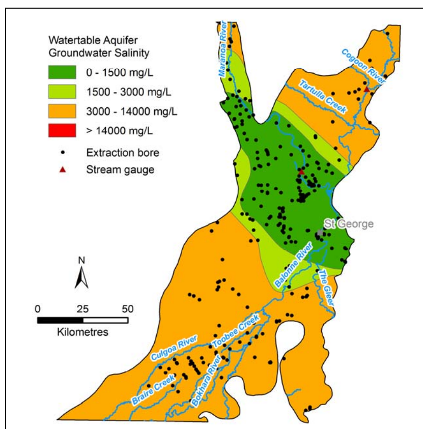
Figure 16. St George Alluvium: Condamine-Balonne SDL area watertable aquifer salinity distribution, from the shallow salinity layer of the MDBA Basin in a Box dataset (MDBA, 2000)
