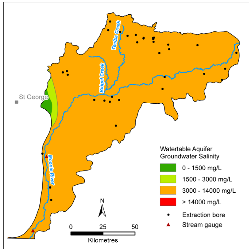
Figure 10. Sediments Above GAB: Moonie watertable aquifer salinity distribution, from the shallow salinity layer of the MDBA Basin in a Box dataset (MDBA, 2000)
