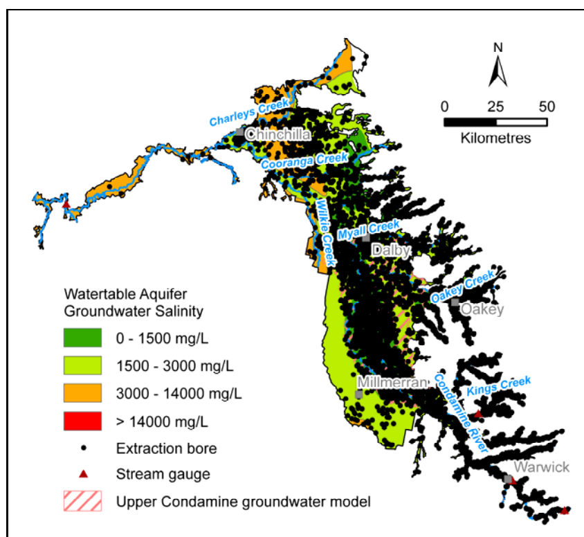
Figure 1. Upper Condamine Alluvium watertable aquifer salinity distribution, from the shallow salinity layer of the MDBA Basin in a Box dataset (MDBA, 2000)
