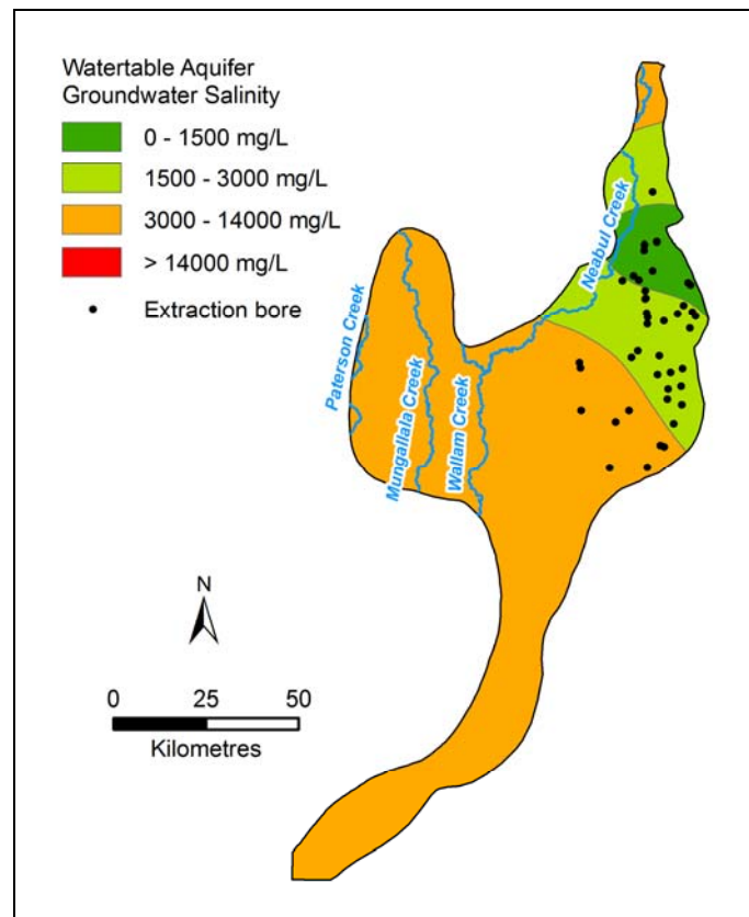
Figure 17. St George Alluvium: Warrego-Paroo-Nebine SDL area watertable aquifer salinity distribution, from the shallow salinity layer of the MDBA Basin in a Box dataset (MDBA, 2000)
