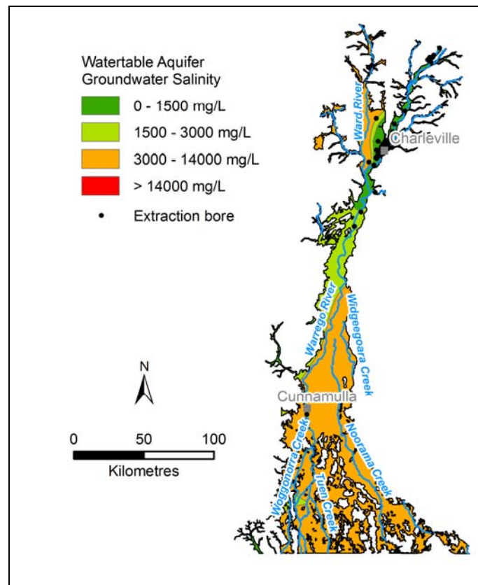
Figure 14. Warrego Alluvium watertable aquifer salinity distribution, from the shallow salinity layer of the MDBA Basin in a Box dataset (MDBA, 2000)
