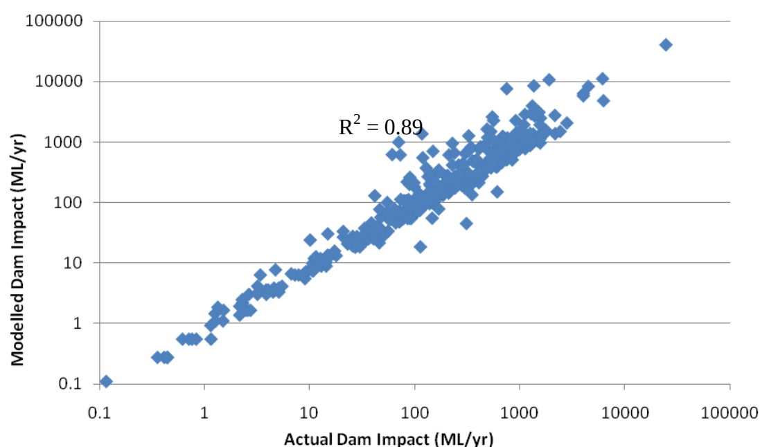
Figure 32: Actual impact versus modelled impact from Relationship 1
