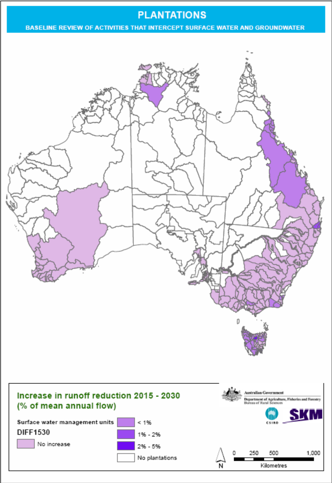
Figure 17: Distribution of SWMAs where plantations potentially impact on hydrology—projected increase in the impact of plantations 2015–2030
