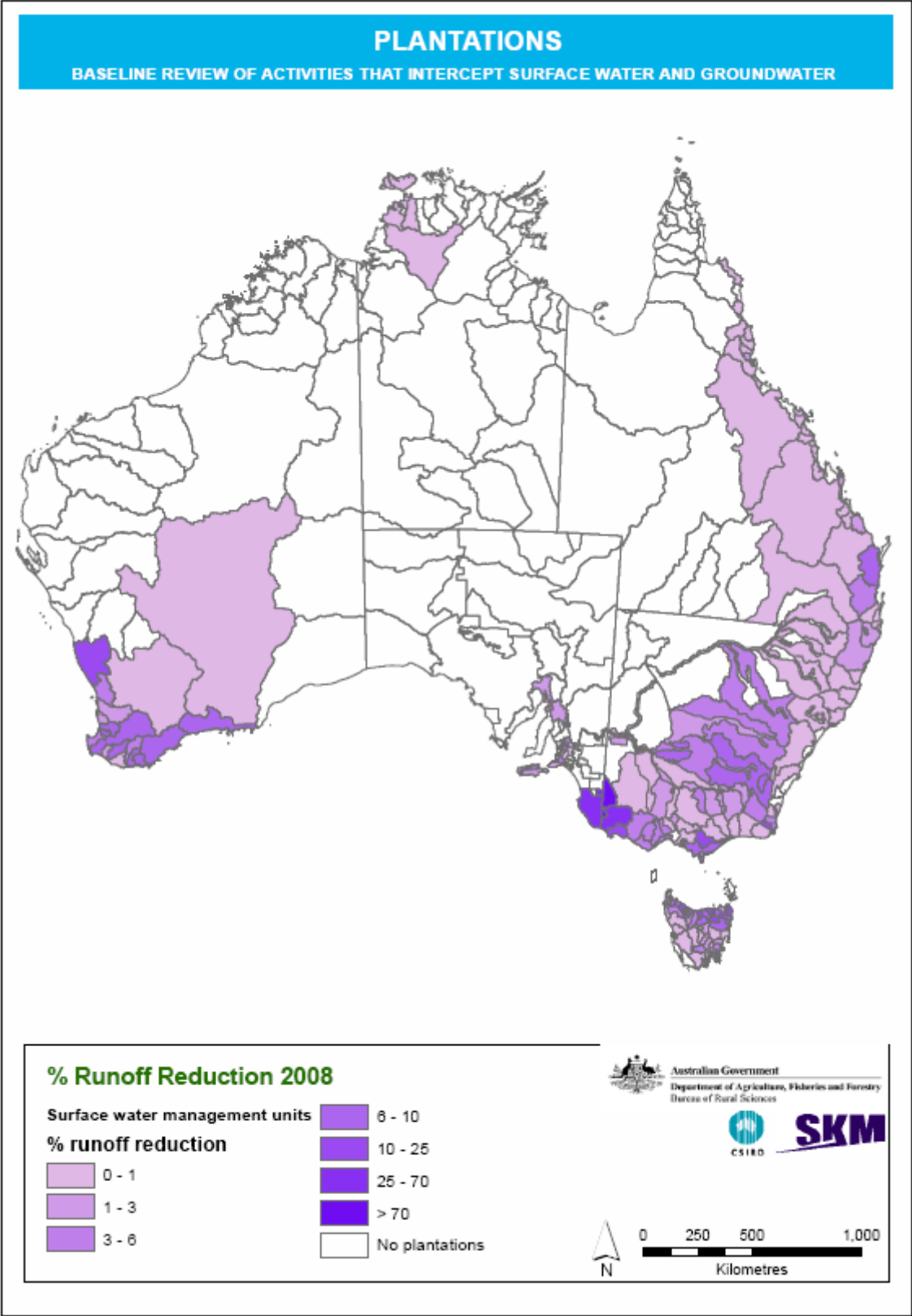
Figure 15: Distribution of SWMAs where plantations potentially impact on hydrology—percentage runoff reduction against mean annual flow
