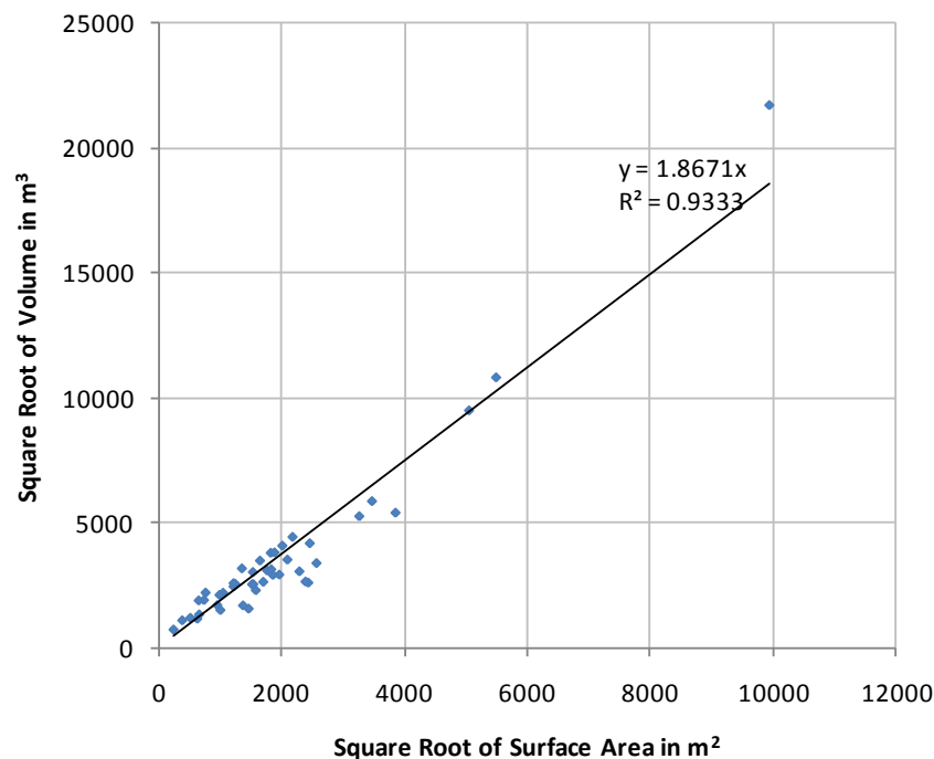
Figure 27: Relationship between volume and surface area of floodplain harvesting dams in the Lower Balonne basin, Queensland
