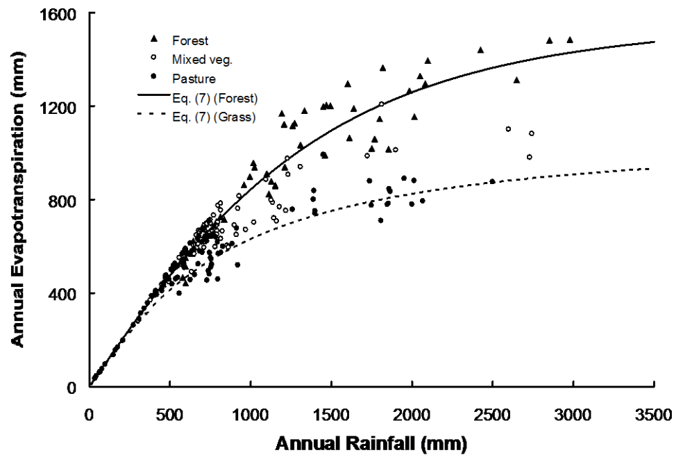
Figure 48: Relationship between annual evapotranspiration and rainfall for different broad vegetation types
