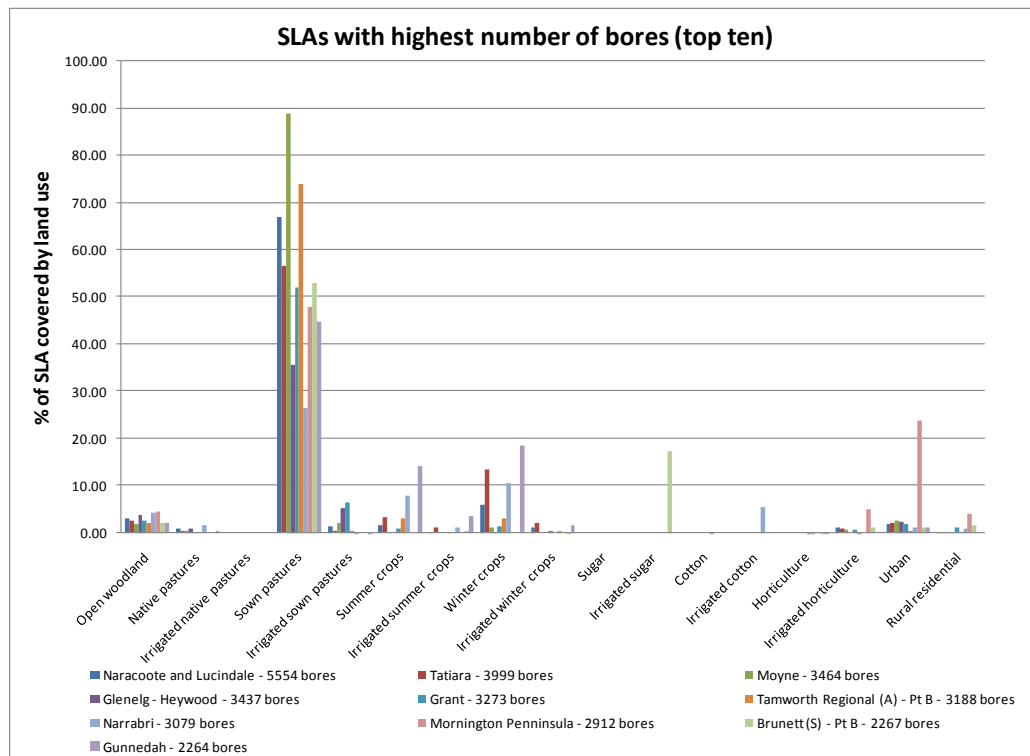
Figure 38: Predominant land use types within SLAs with highest number of bores
