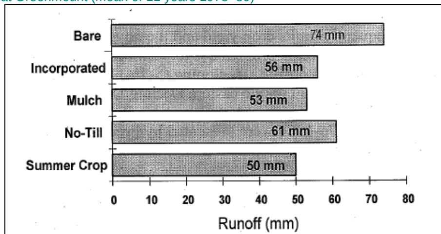
Figure 25: Mean annual runoff for five management options during the summer fallow period at Greenmount (mean of 11 years 1978–89)
