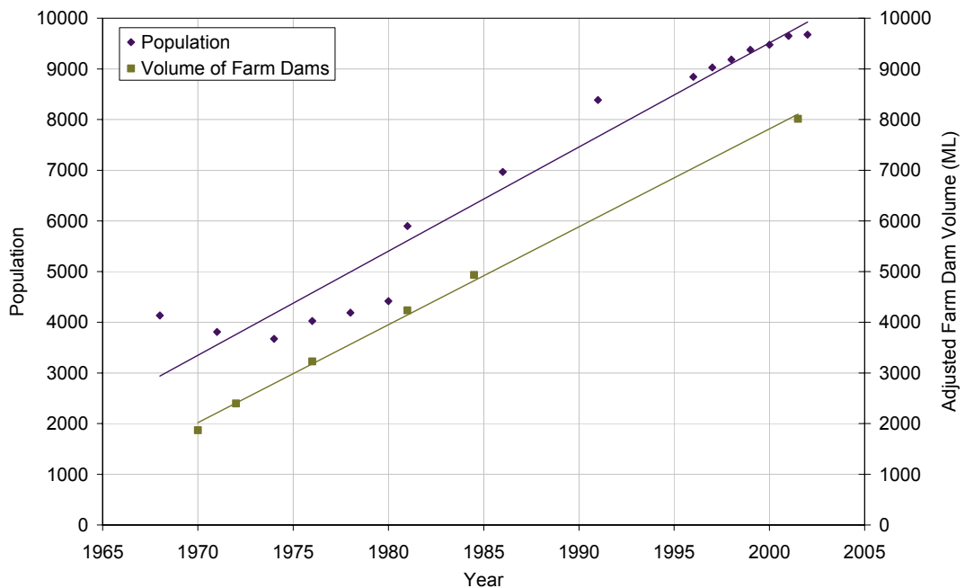
■ Figure 5-14 Time series of population and total estimated storage volume of farm dams in the Moorabool River Catchment for 1968 through 2002.
