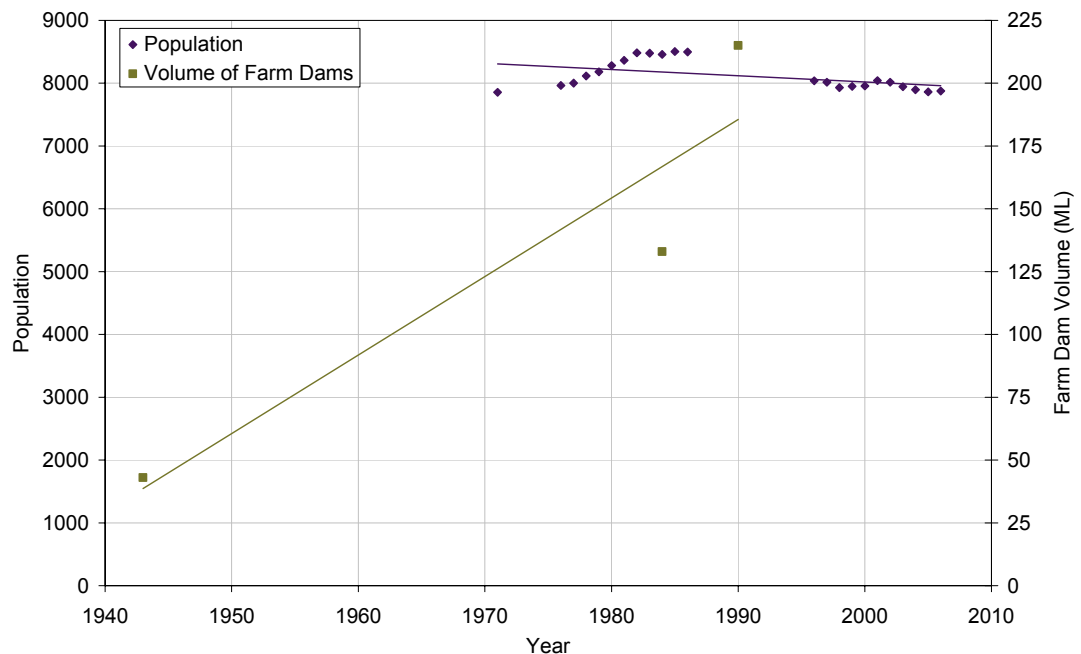
■ Figure 5-13 Population and estimated farm dam volume in the Warrah Creek @ Old Warrah Catchment in NSW
