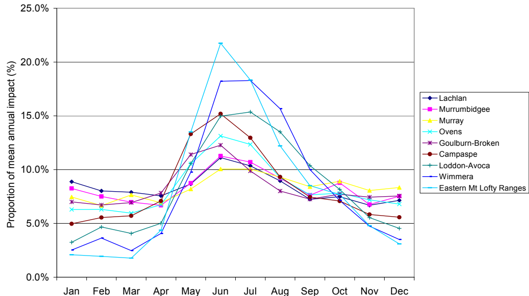
■ Figure 8-3 Proportion of mean annual impact that occurs in each month of the calendar year for reporting regions that are generally in the south of the MDB
