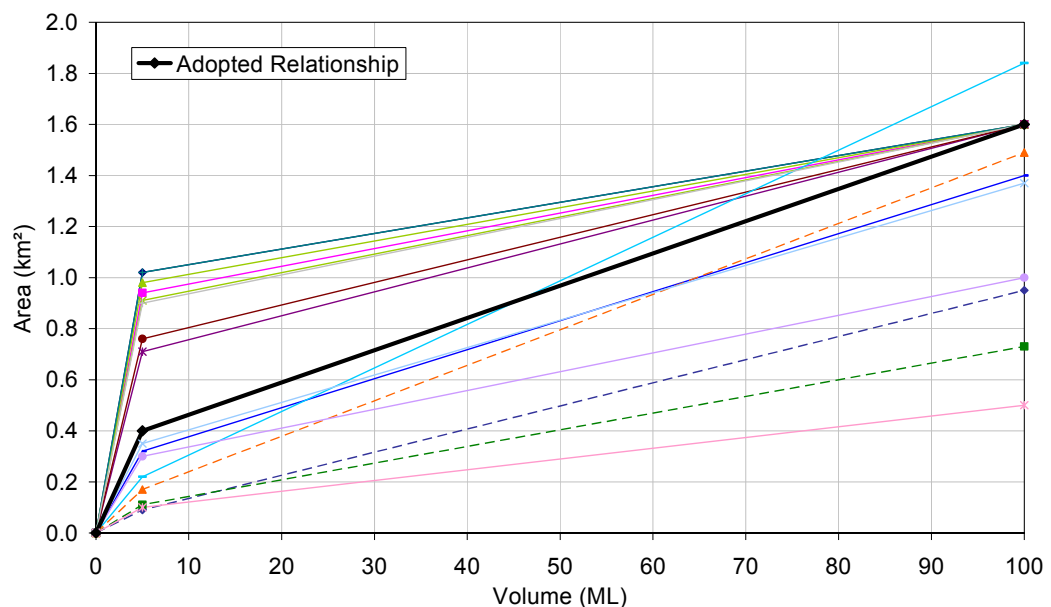
■ Figure 7-2 Comparison between the volume-catchment area relationship adopted for this study (black bold line) and relationships derived from several other similar studies from catchments in Victoria and South Australia.
