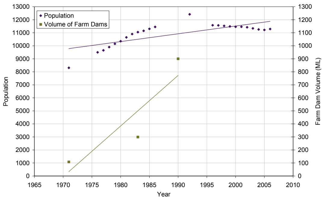
■ Figure 5-11 Population and estimated farm dam volume in the Swamp Oak Creek @ Limbri Catchment in NSW
