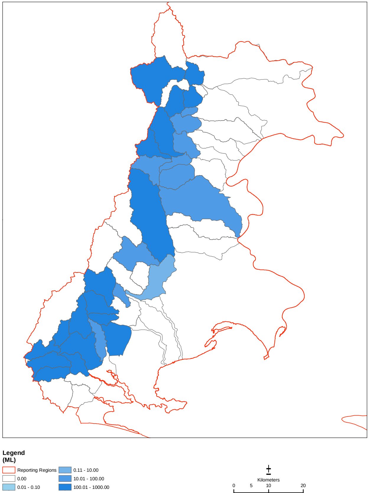
n Figure 5-4 Upper limit on future growth in farm dam volume for modelling subcatchments in the EMLR, based on assumed farm dam development policy, existing farm dam volumes and existing and projected areas of plantation forestry.
