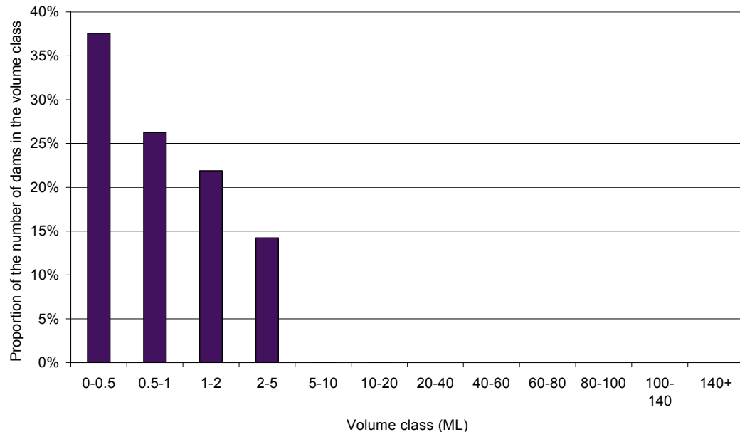
■ Figure 6-3 Probability distribution of existing storage volume of stock and domestic farm dams (less than 5 ML capacity), by farm dam volume, for Victoria
