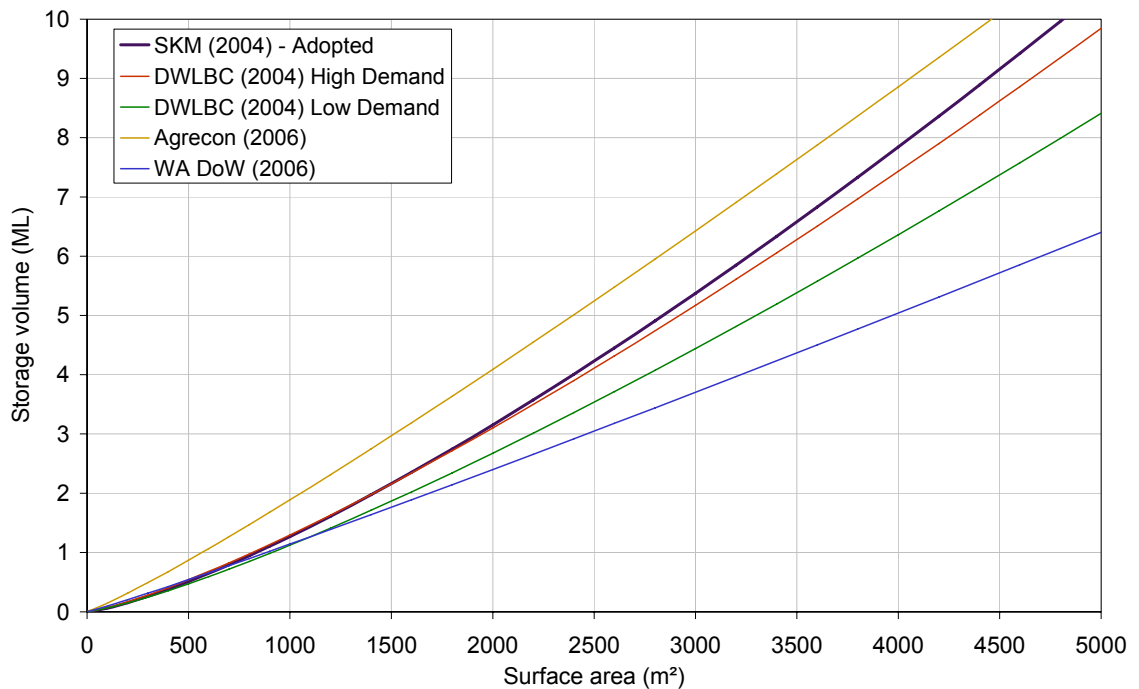
■ Figure 4-1 Surface area versus storage volume relationships from studies in literature, showing only surface areas up to 5000 m² and volumes up to 10 ML
